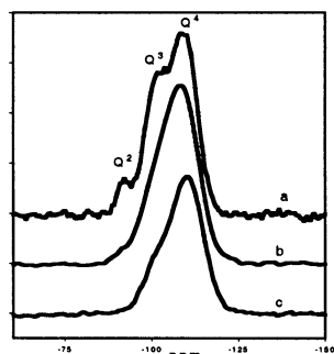
Figure 3. ^{29}\text{Si} MAS NMR spectra of (a) parent MCF, (b) NaY-coated MCF, and (c) ZSM-5-coated MCF.
