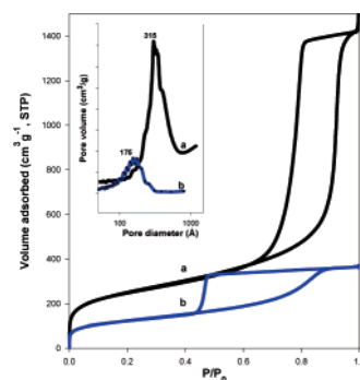
Figure 1. N 2 adsorption/desorption isotherms at –196 °C and BdB-FHH pore diameter distributions calculated from the adsorption branch of the isotherm (inset) for (a) parent MCF and (b) ZSM-coated MCF.
