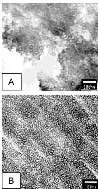
Figure 2. TEM image of (A) parent MCF and (B) ZSM-5-coated MCF.
